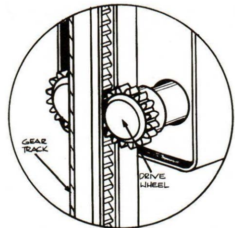
DRIVE WHEEL DETAIL
