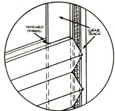
NOTCHED FABRIC DETAIL
